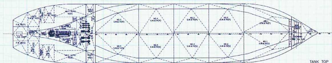
TANK TOP
