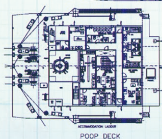
POOP DECK
