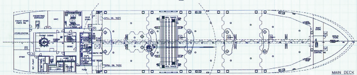
MAIN DECK
